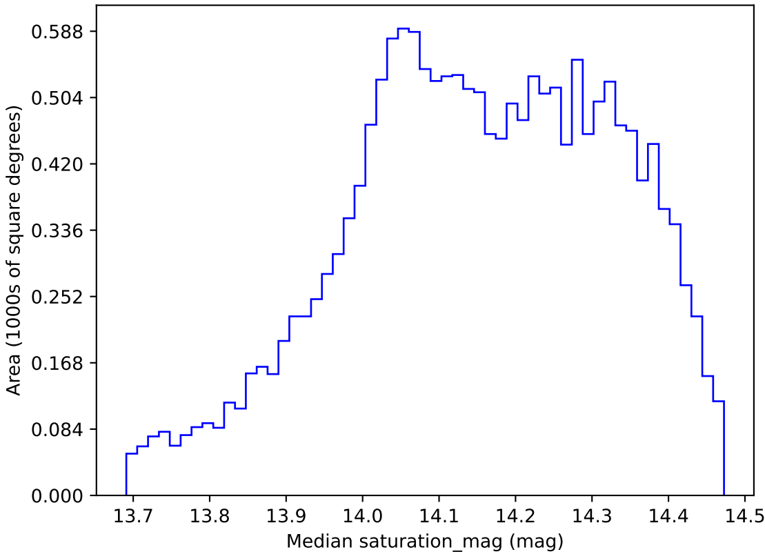
ddf_loaded_fl4_v3.4_10yrs WFD all bands: Median saturation_mag
