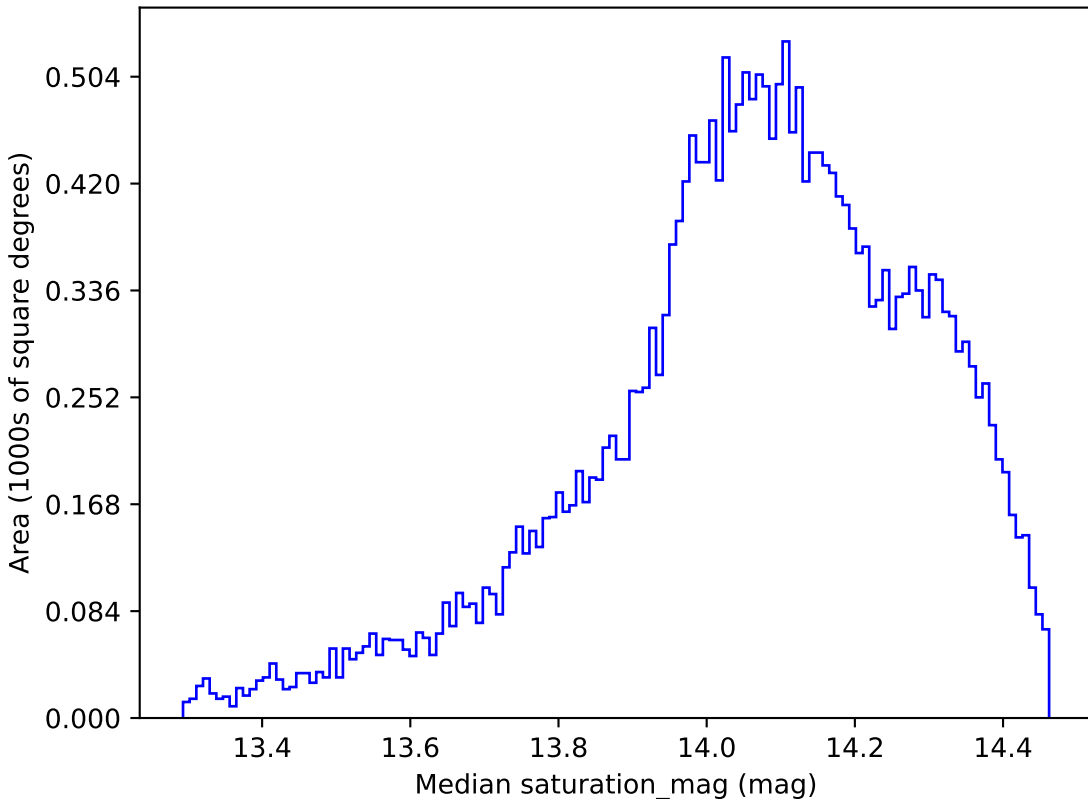
ddf_loaded_fl4_v3.4_10yrs All sky z band: Median saturation_mag
