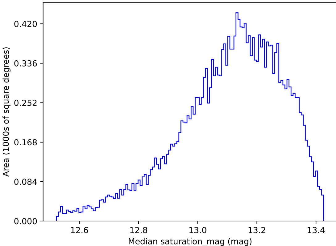
ddf_loaded_fl4_v3.4_10yrs All sky y band: Median saturation_mag
