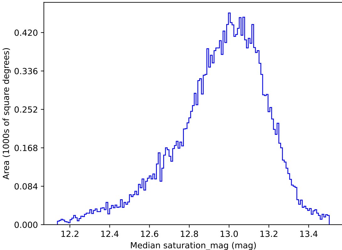
ddf_loaded_fl4_v3.4_10yrs All sky u band: Median saturation_mag
