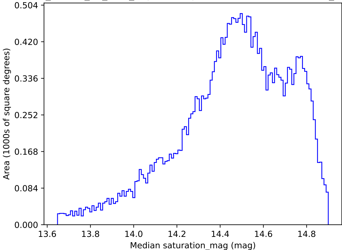
ddf_loaded_fl4_v3.4_10yrs All sky i band: Median saturation_mag
