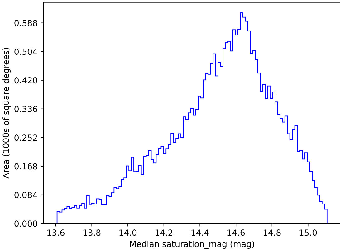
ddf_loaded_fl4_v3.4_10yrs All sky g band: Median saturation_mag
