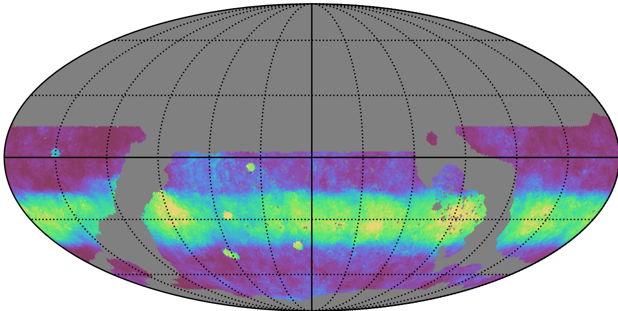
ddf_loaded_fl4_v3.4_10yrs WFD z band: Median normairmass
