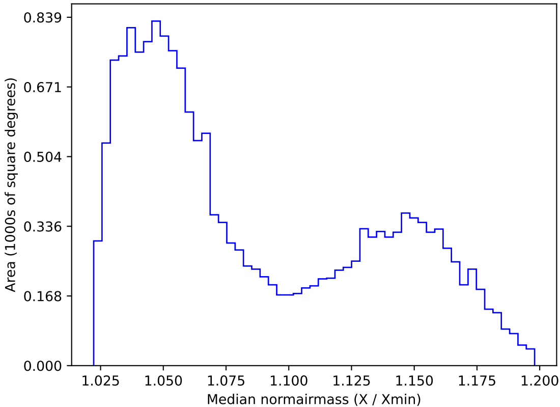
ddf_loaded_fl4_v3.4_10yrs WFD z band: Median normairmass
