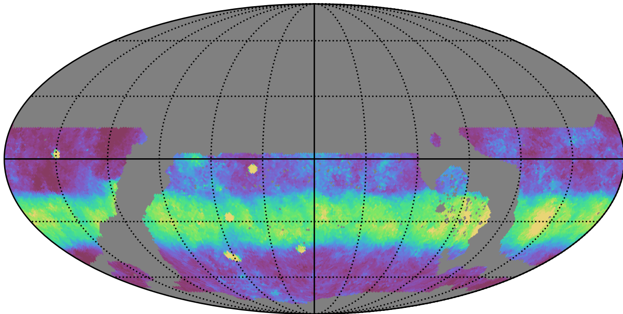
ddf_loaded_fl4_v3.4_10yrs WFD y band: Median normairmass
