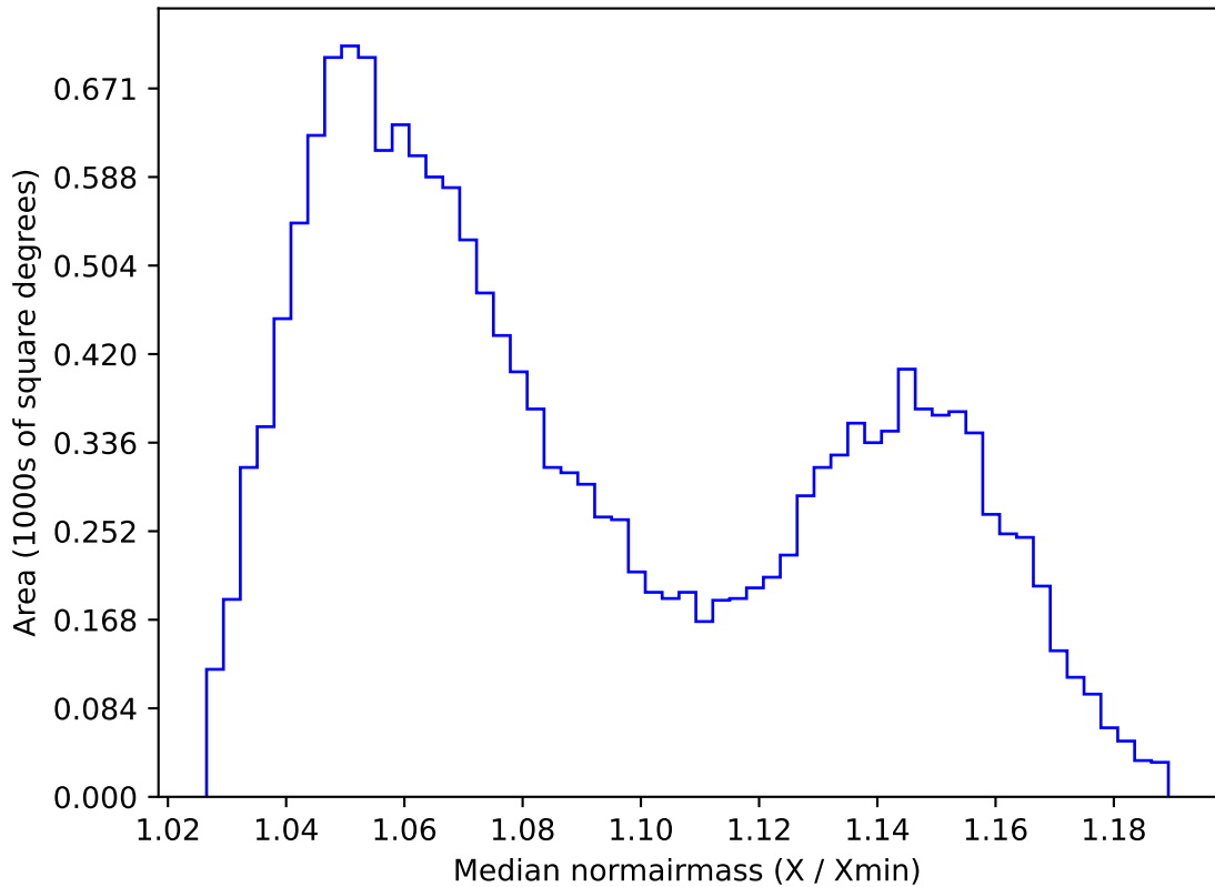
ddf_loaded_fl4_v3.4_10yrs WFD y band: Median normairmass
