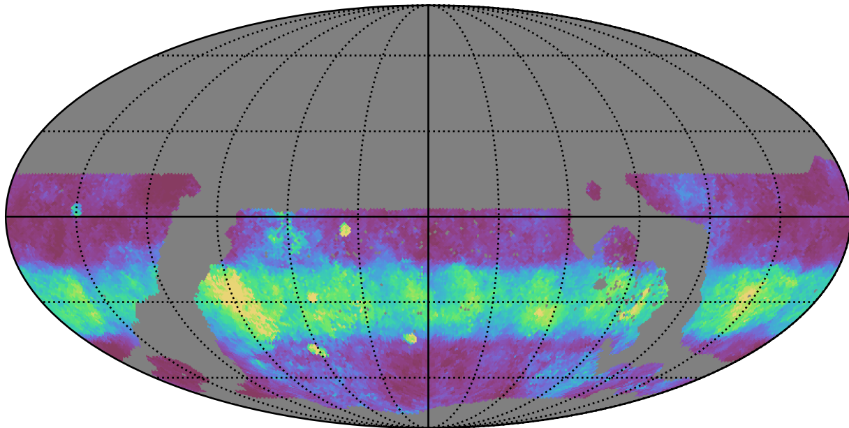
ddf_loaded_fl4_v3.4_10yrs WFD u band: Median normairmass
