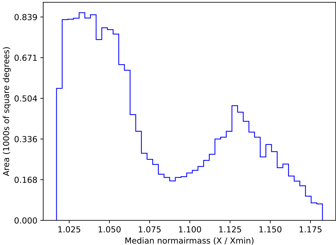
ddf_loaded_fl4_v3.4_10yrs WFD r band: Median normairmass
