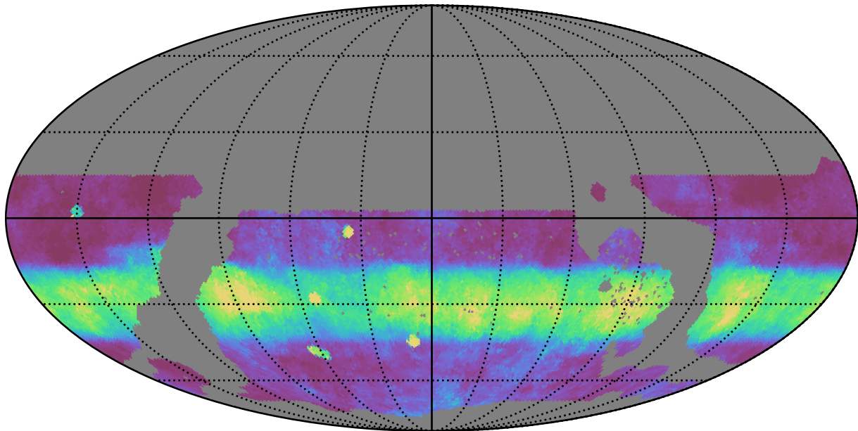
ddf_loaded_fl4_v3.4_10yrs WFD i band: Median normairmass
