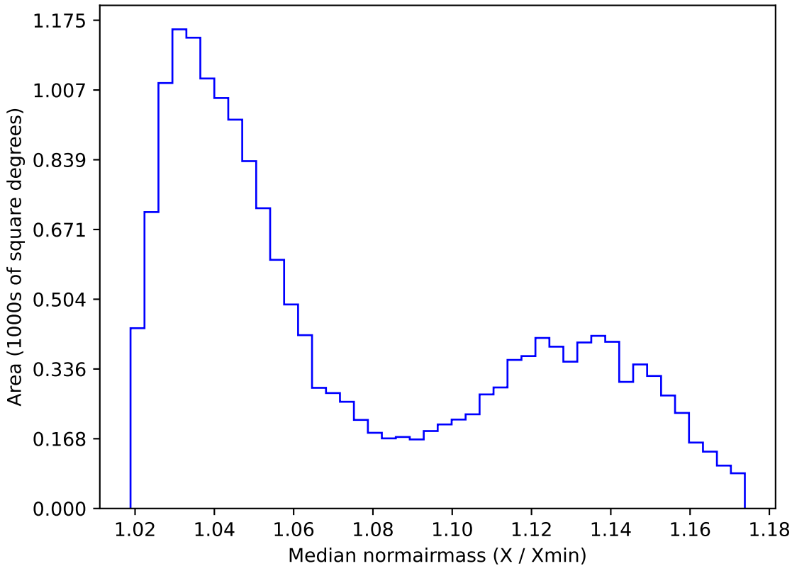
ddf_loaded_fl4_v3.4_10yrs WFD i band: Median normairmass
