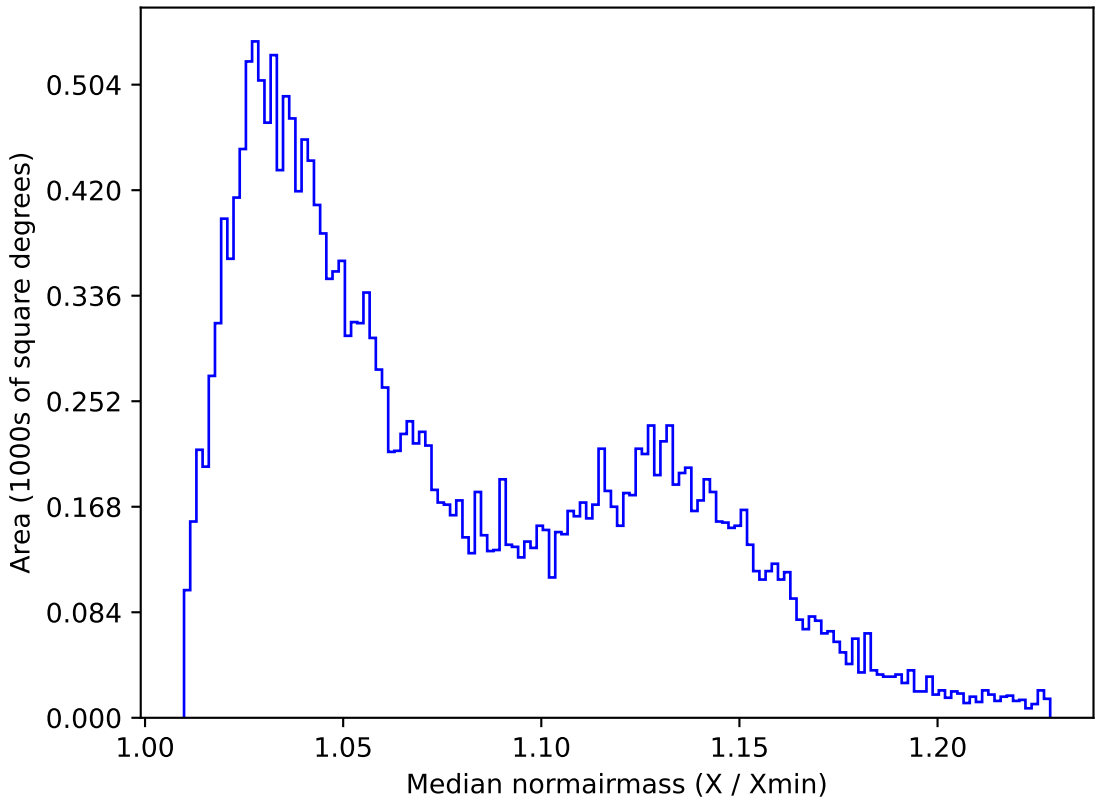
ddf_loaded_fl4_v3.4_10yrs All sky u band: Median normairmass
