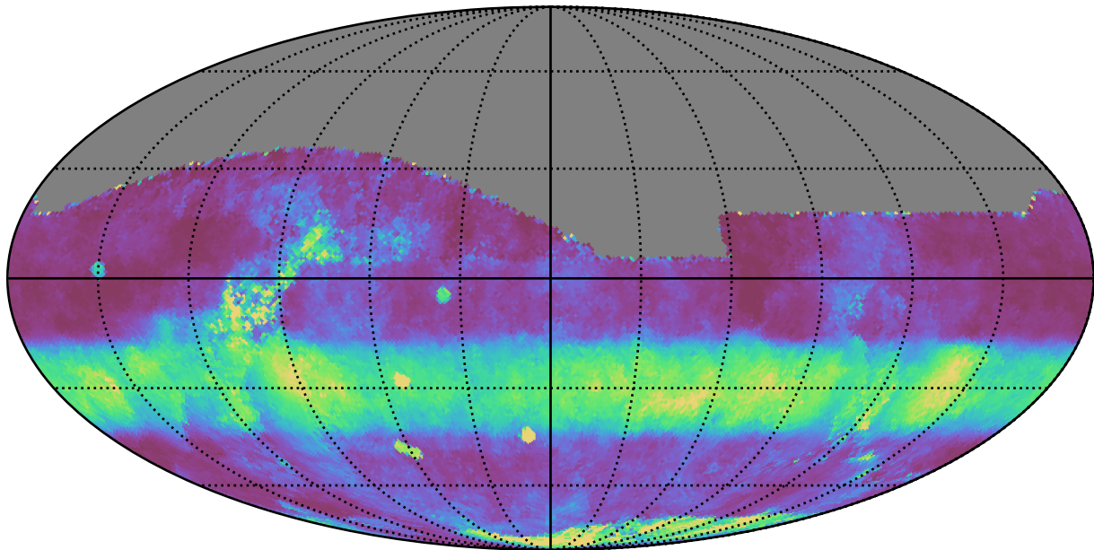
ddf_loaded_fl4_v3.4_10yrs All sky r band: Median normairmass
