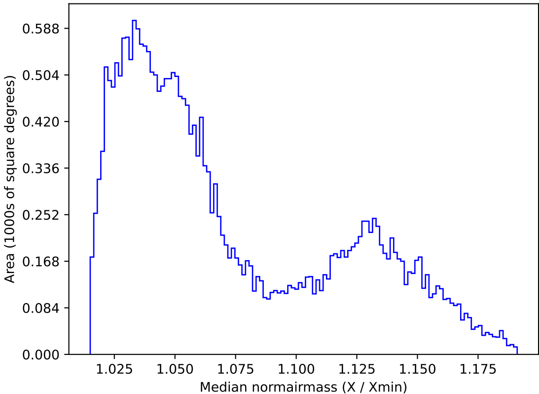
ddf_loaded_fl4_v3.4_10yrs All sky r band: Median normairmass
