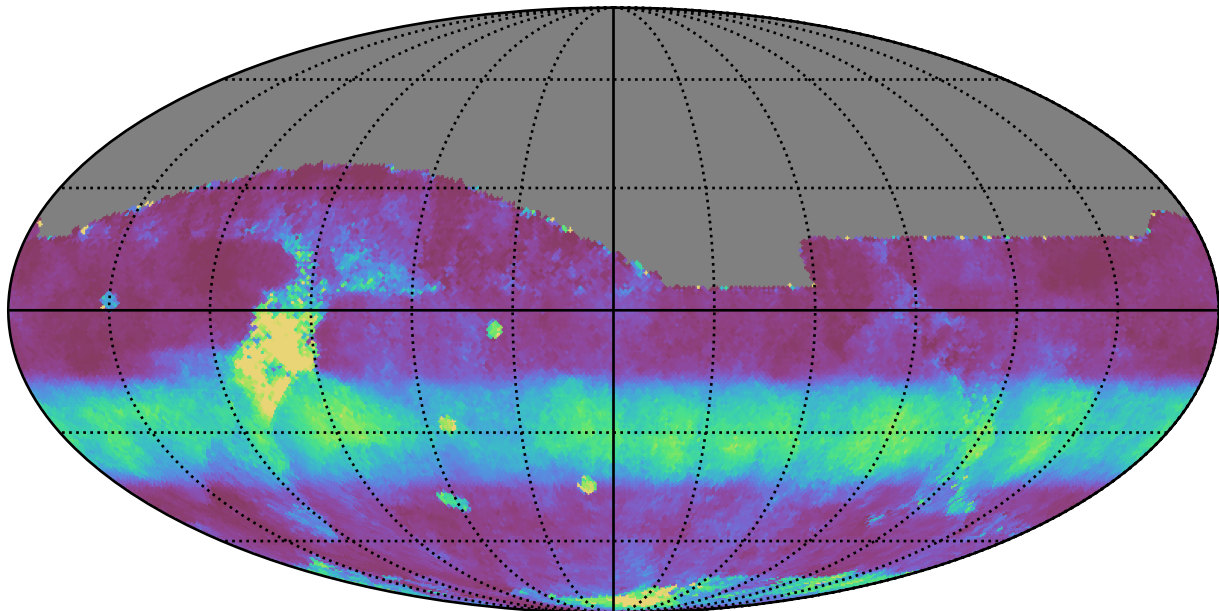
ddf_loaded_fl4_v3.4_10yrs All sky i band: Median normairmass
