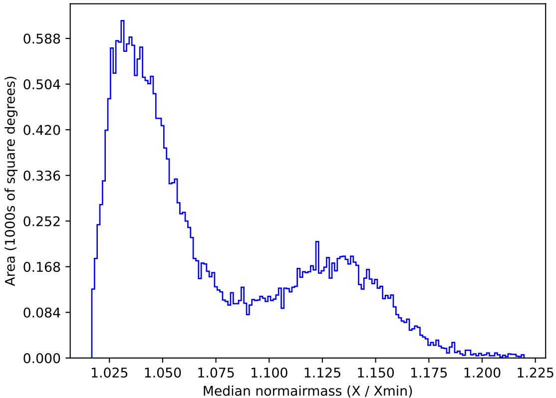
ddf_loaded_fl4_v3.4_10yrs All sky i band: Median normairmass
