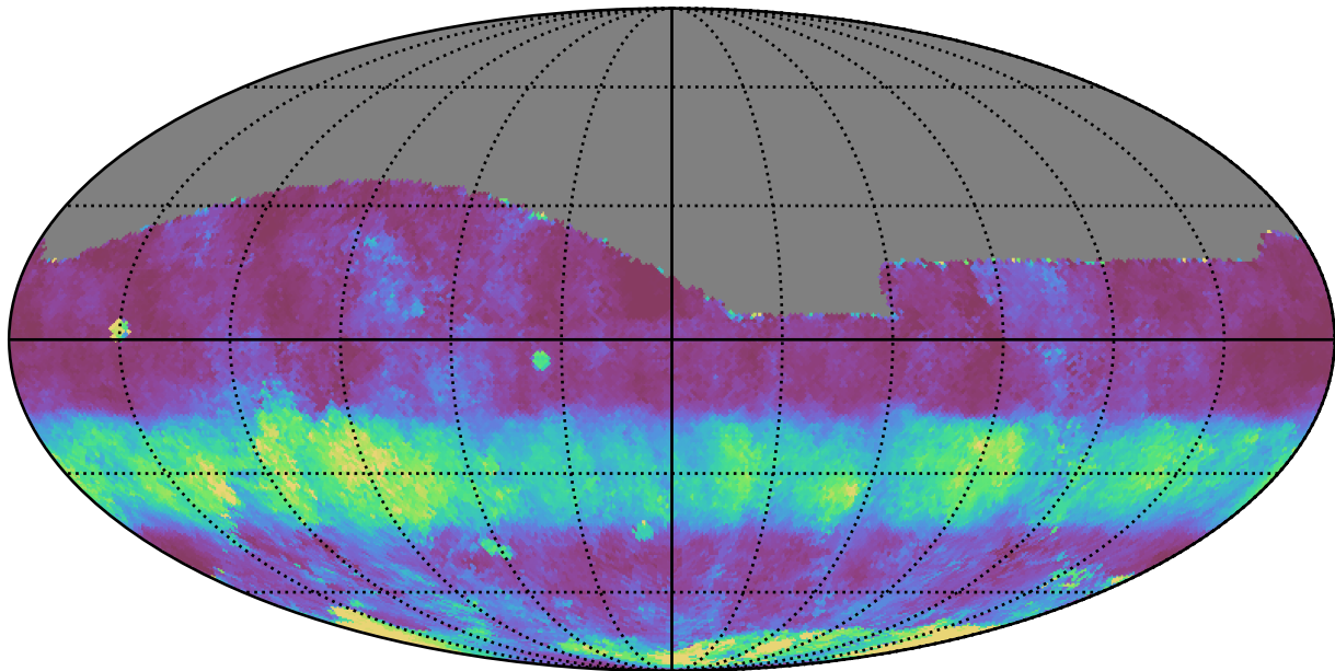
ddf_loaded_fl4_v3.4_10yrs All sky g band: Median normairmass
