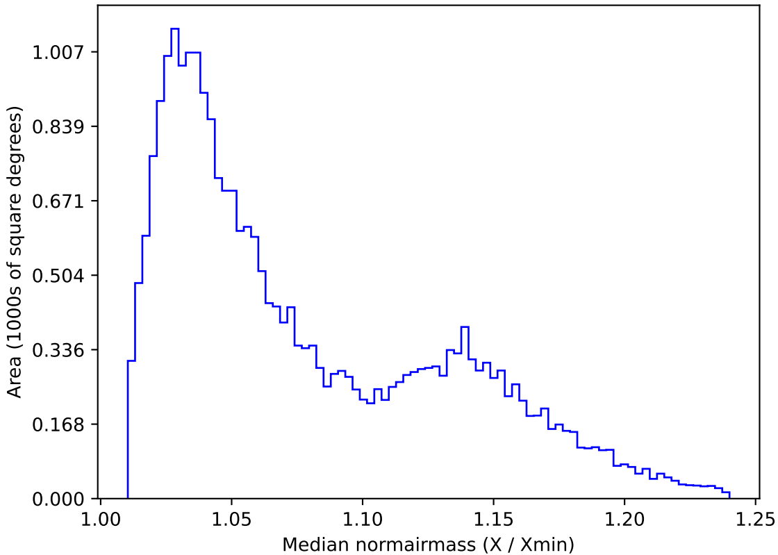
ddf_loaded_fl4_v3.4_10yrs All sky g band: Median normairmass
