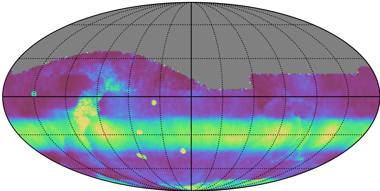
ddf_loaded_fl4_v3.4_10yrs All sky all bands: Median normairmass
