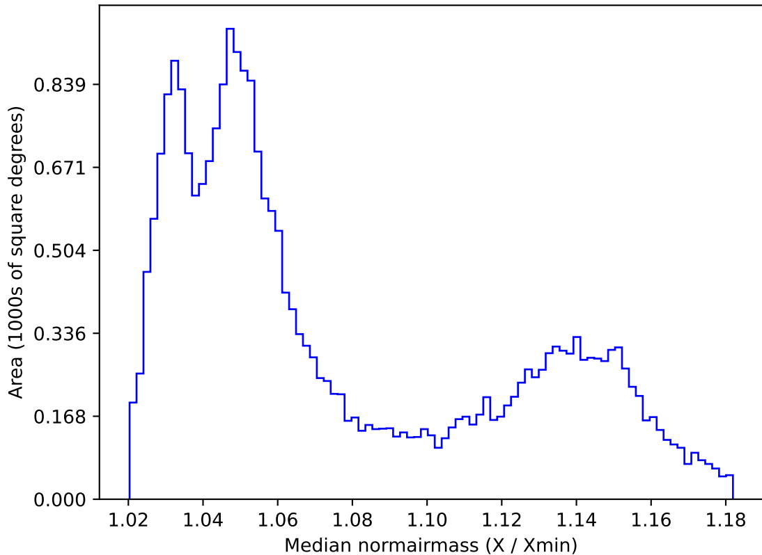
ddf_loaded_fl4_v3.4_10yrs All sky all bands: Median normairmass
