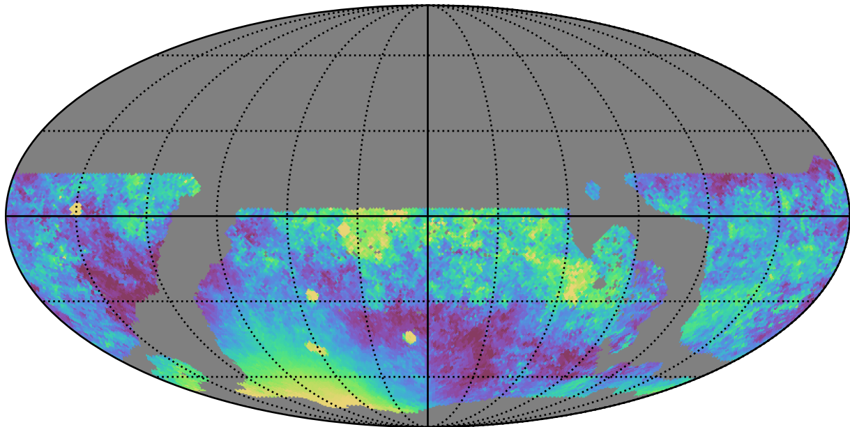
ddf_loaded_fl4_v3.4_10yrs WFD z band: Median moonDistance
