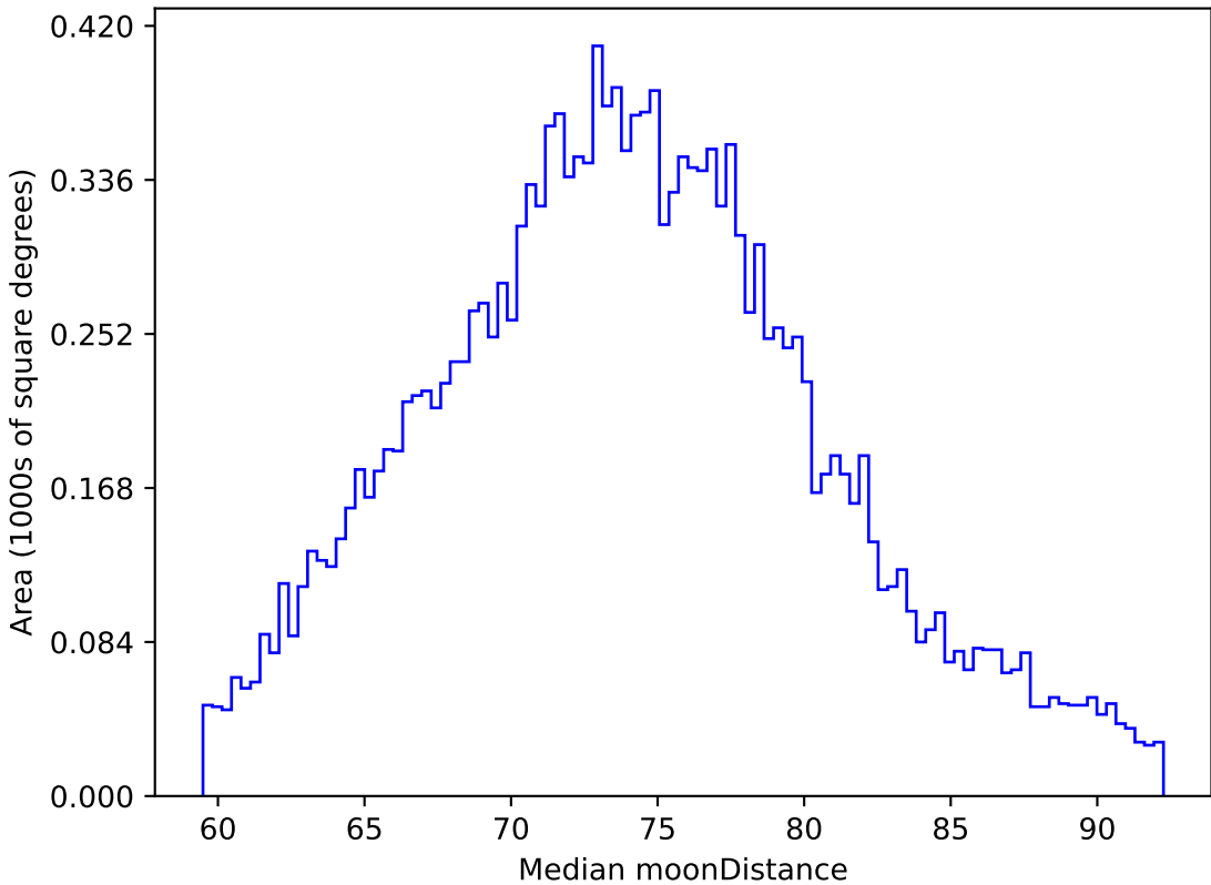
ddf_loaded_fl4_v3.4_10yrs WFD z band: Median moonDistance
