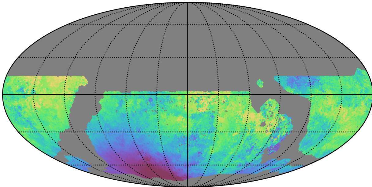
ddf_loaded_fl4_v3.4_10yrs WFD u band: Median moonDistance
