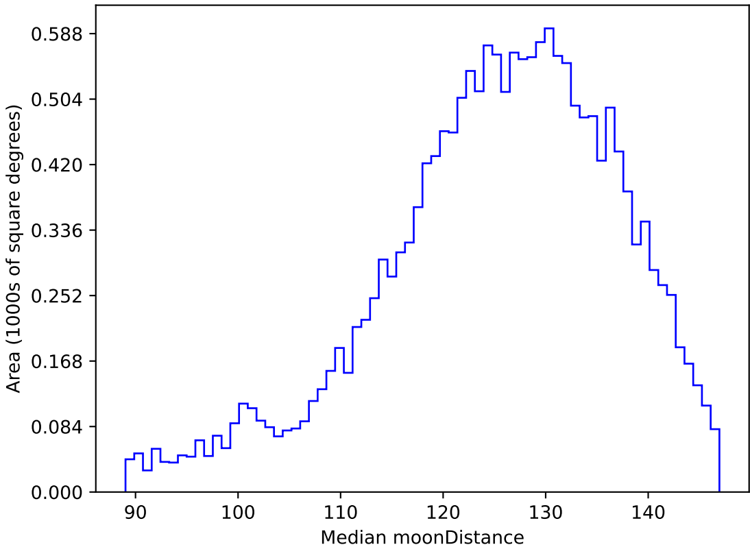
ddf_loaded_fl4_v3.4_10yrs WFD u band: Median moonDistance
