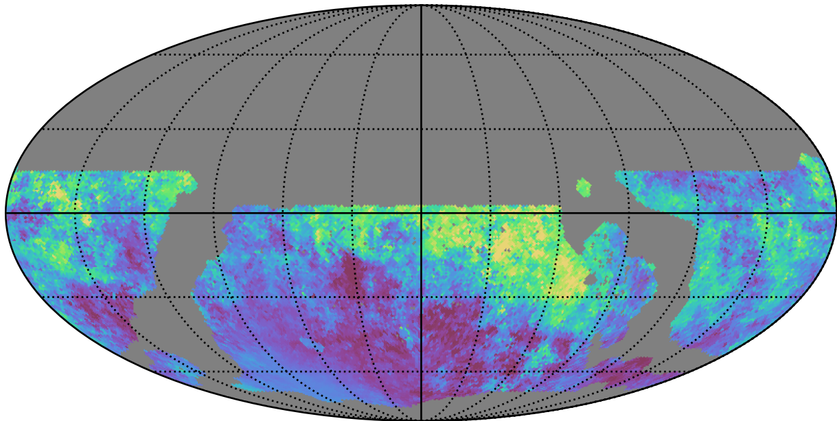
ddf_loaded_fl4_v3.4_10yrs WFD i band: Median moonDistance
