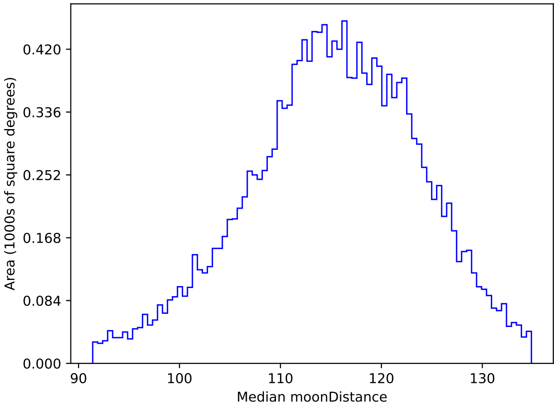
ddf_loaded_fl4_v3.4_10yrs WFD g band: Median moonDistance
