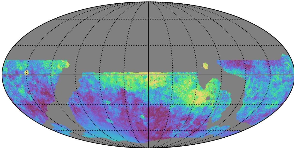
ddf_loaded_fl4_v3.4_10yrs WFD all bands: Median moonDistance
