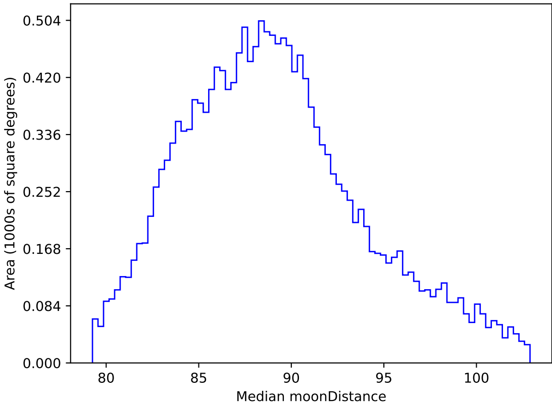
ddf_loaded_fl4_v3.4_10yrs WFD all bands: Median moonDistance
