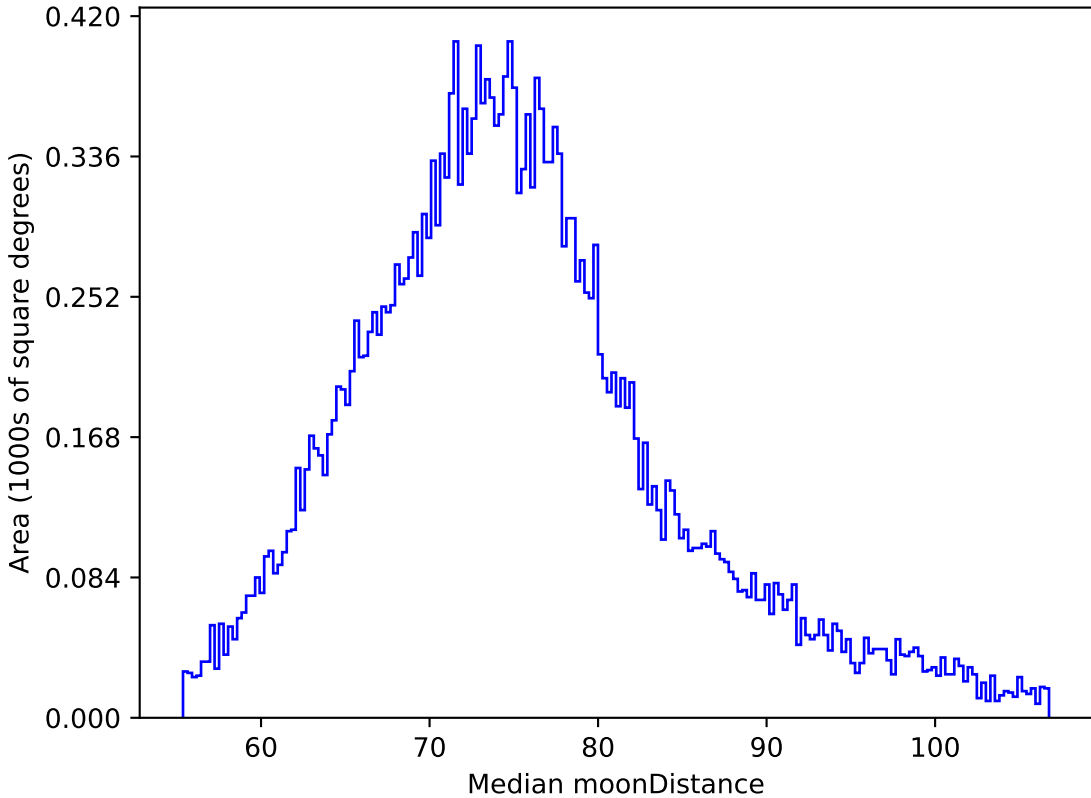
ddf_loaded_fl4_v3.4_10yrs All sky z band: Median moonDistance
