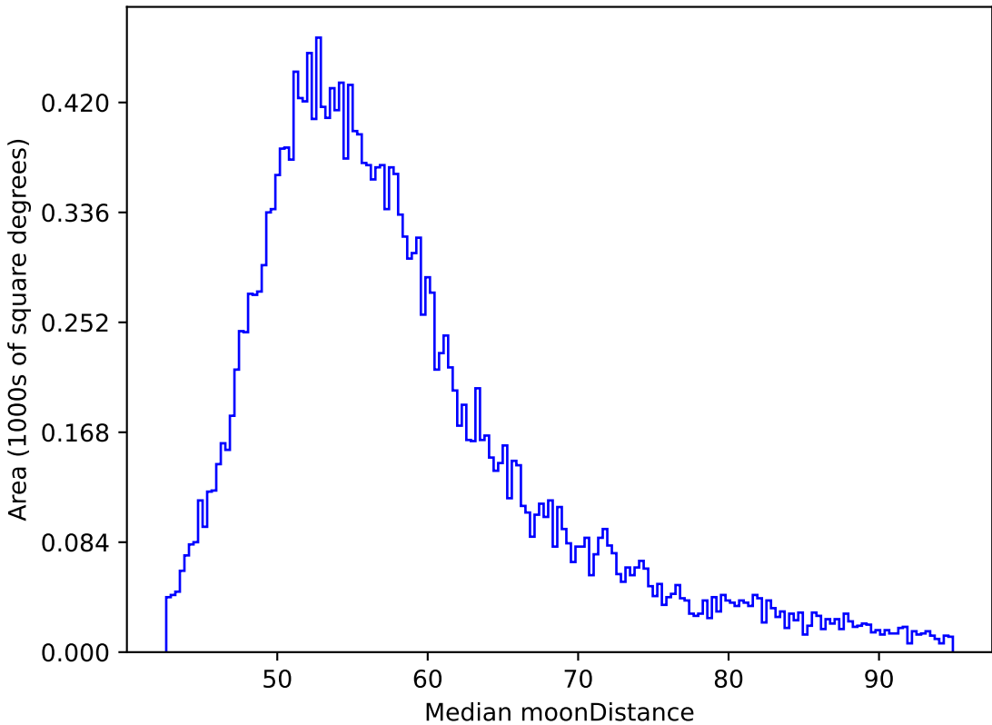
ddf_loaded_fl4_v3.4_10yrs All sky y band: Median moonDistance
