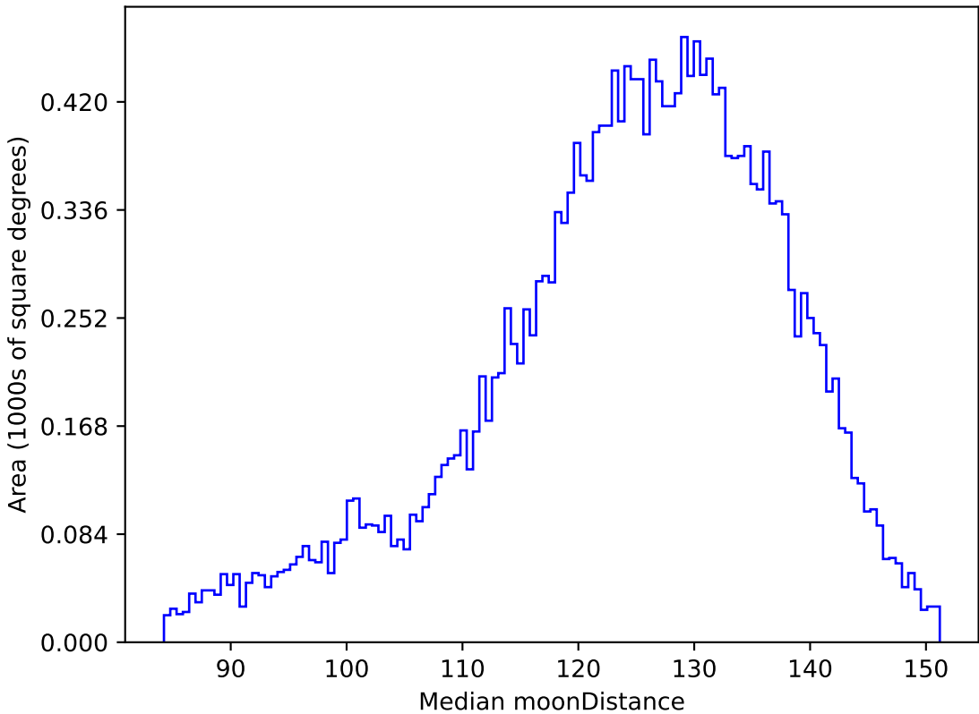
ddf_loaded_fl4_v3.4_10yrs All sky u band: Median moonDistance
