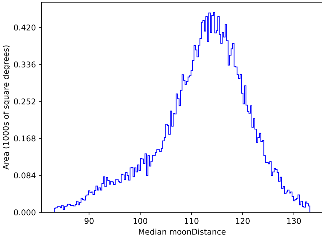
ddf_loaded_fl4_v3.4_10yrs All sky r band: Median moonDistance
