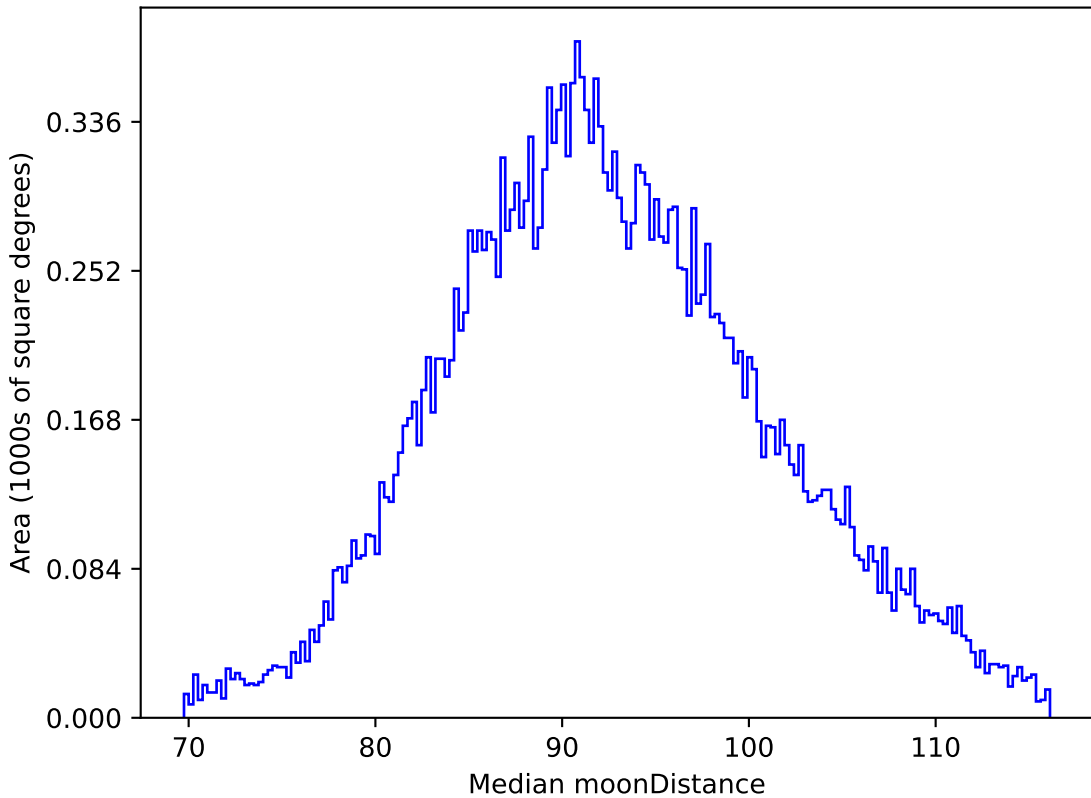
ddf_loaded_fl4_v3.4_10yrs All sky i band: Median moonDistance
