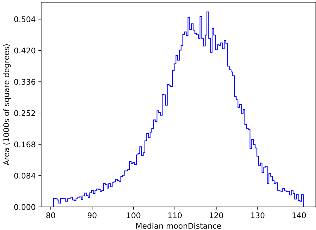
ddf_loaded_fl4_v3.4_10yrs All sky g band: Median moonDistance
