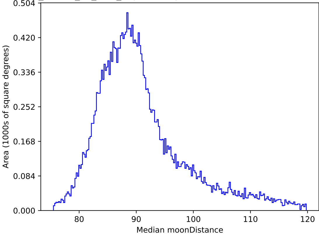
ddf_loaded_fl4_v3.4_10yrs All sky all bands: Median moonDistance
