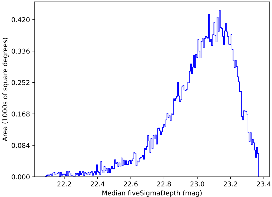
ddf_loaded_fl4_v3.4_10yrs Yr 1 z band: Median fiveSigmaDepth
