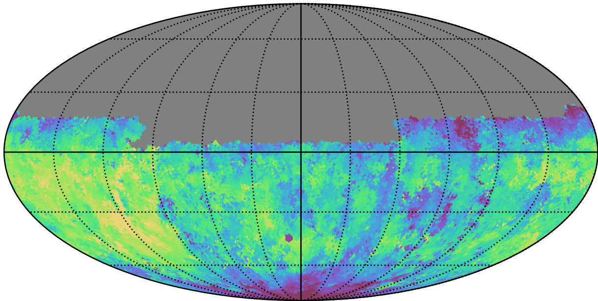
ddf_loaded_fl4_v3.4_10yrs Yr 1 u band: Median fiveSigmaDepth
