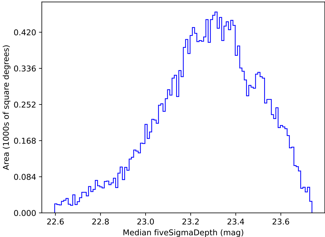
ddf_loaded_fl4_v3.4_10yrs Yr 1 u band: Median fiveSigmaDepth
