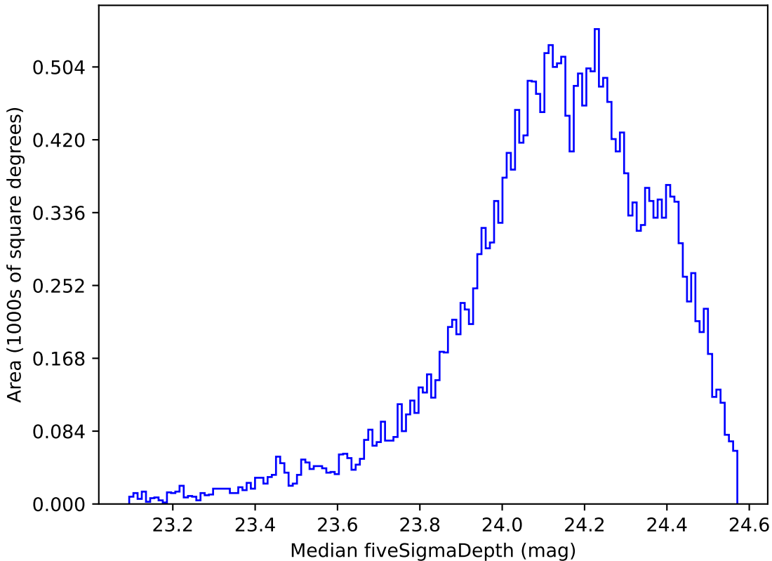
ddf_loaded_fl4_v3.4_10yrs Yr 1 r band: Median fiveSigmaDepth
