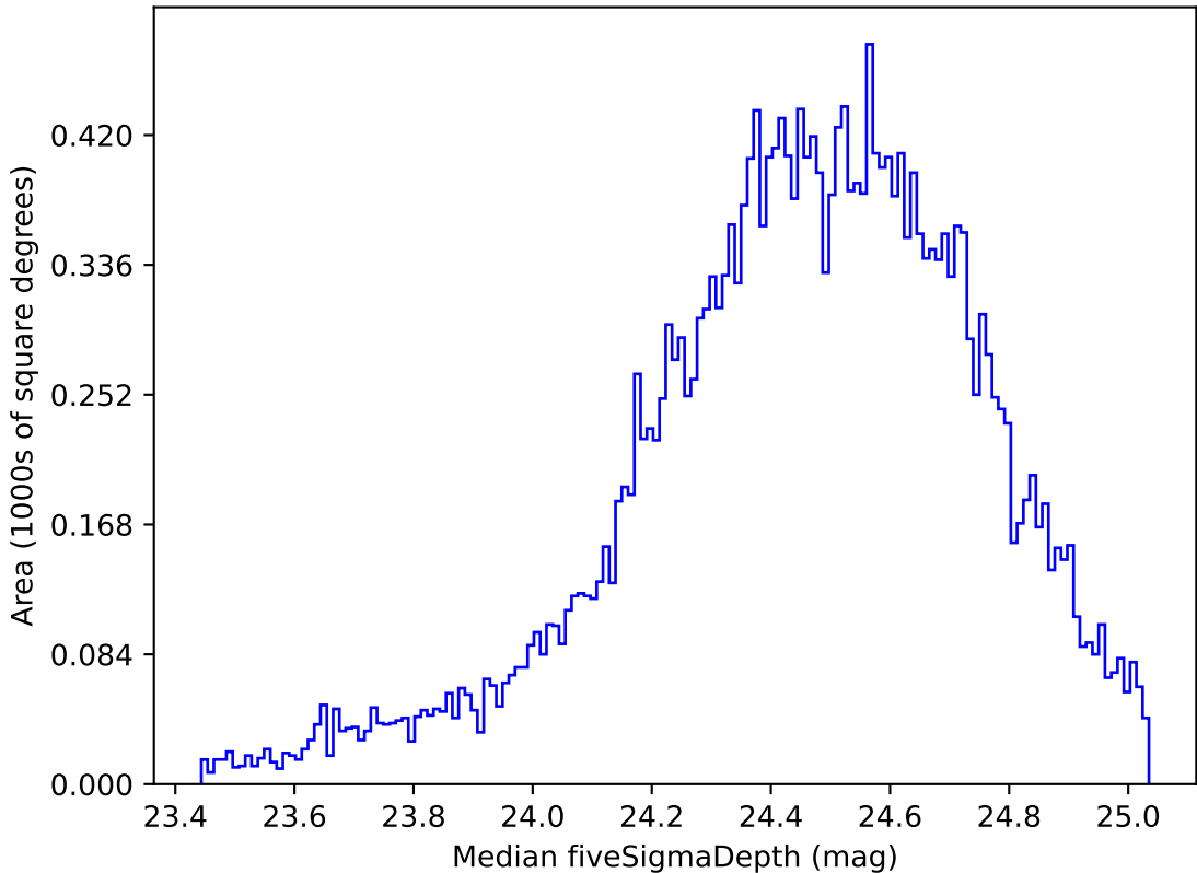
ddf_loaded_fl4_v3.4_10yrs Yr 1 g band: Median fiveSigmaDepth
