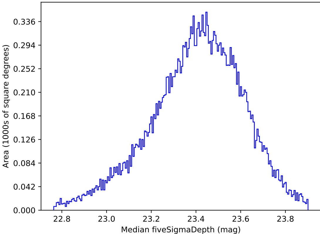
ddf_loaded_fl4_v3.4_10yrs Yr 1 all bands: Median fiveSigmaDepth
