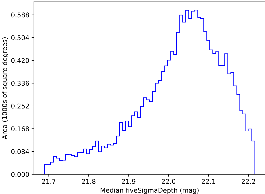
ddf_loaded_fl4_v3.4_10yrs WFD y band: Median fiveSigmaDepth
