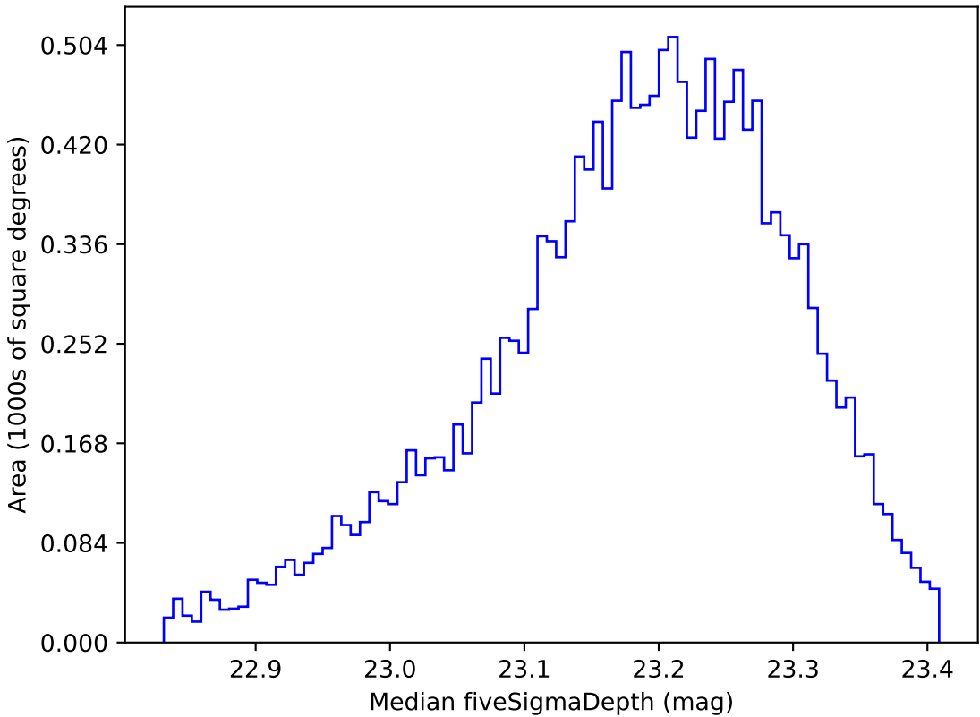
ddf_loaded_fl4_v3.4_10yrs WFD u band: Median fiveSigmaDepth
