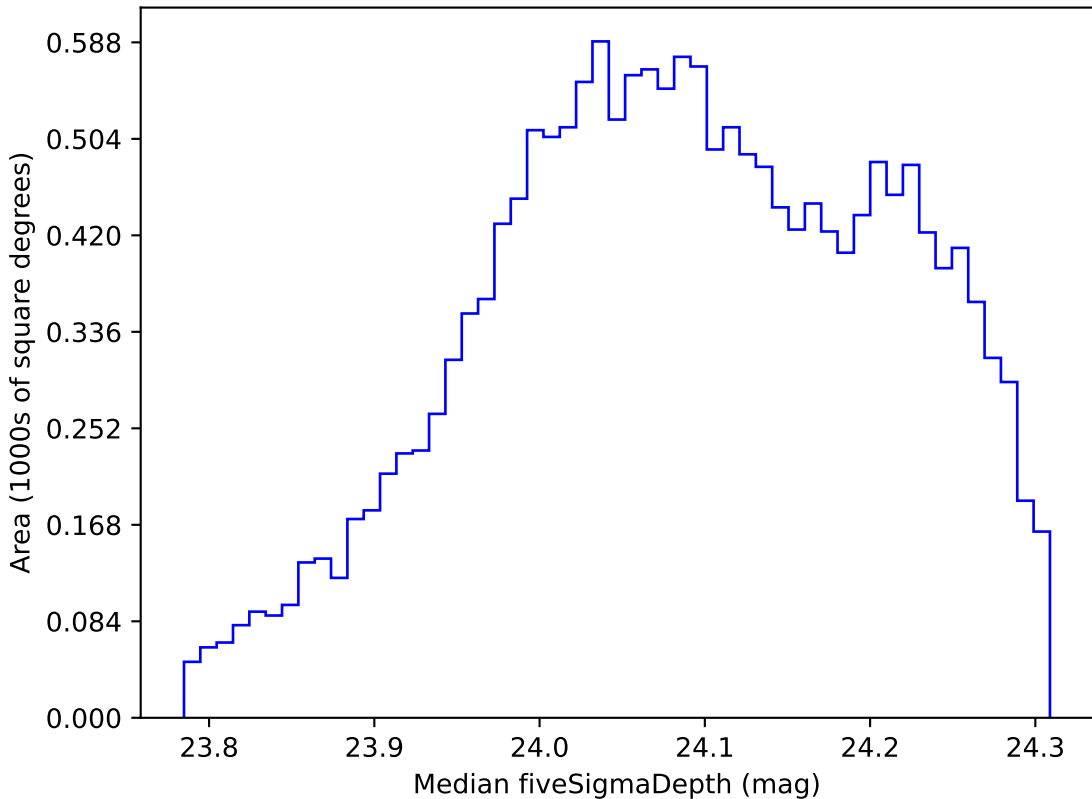
ddf_loaded_fl4_v3.4_10yrs WFD r band: Median fiveSigmaDepth
