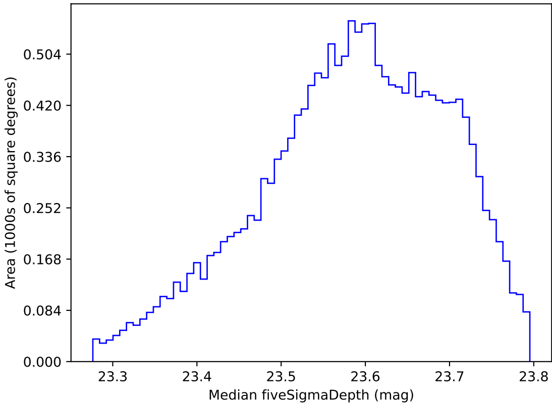
ddf_loaded_fl4_v3.4_10yrs WFD i band: Median fiveSigmaDepth
