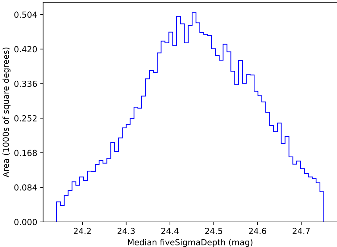
ddf_loaded_fl4_v3.4_10yrs WFD g band: Median fiveSigmaDepth
