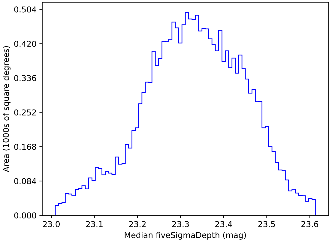
ddf_loaded_fl4_v3.4_10yrs WFD all bands: Median fiveSigmaDepth
